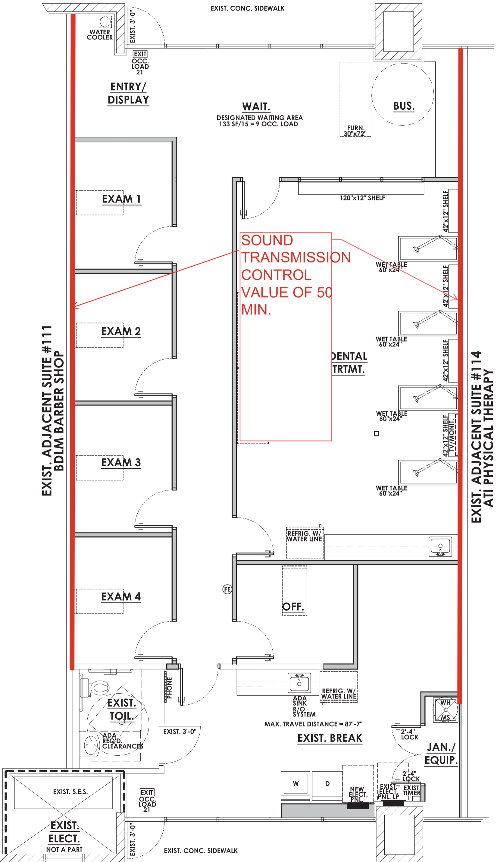
Exhibit 3 | Conceptual Floor Plan
